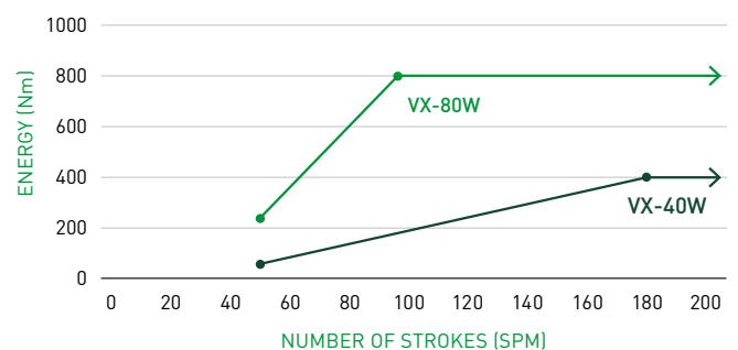
ENERGY DIAGRAM
